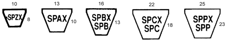
SPC / SPCX SECTION V-BELTS
