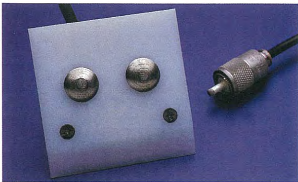
#1986 Bale Sensor — for continuous monitoring during baling. Comes with 30' cable to run from the sensor mounted in the bale chamber to the meter in the cab. May be used with any model, but is recommended to use with Model FX-2000. Also available as 1986/40 with 40' cable for larger balers.
