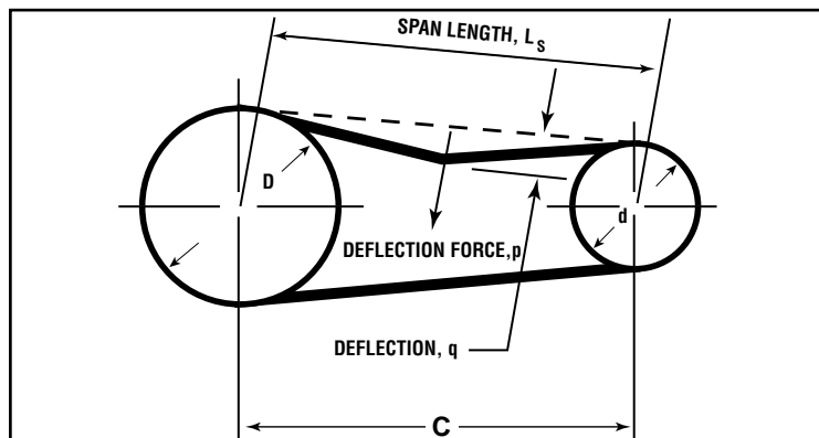
Figure 1 MEASURING DEFLECTION FORCE
