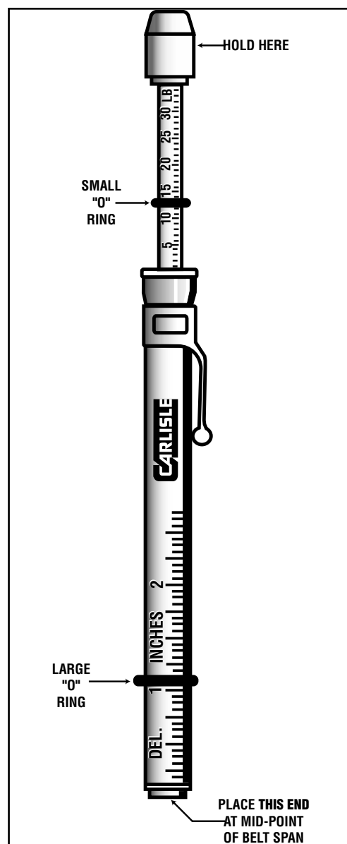
Figure 2 V-BELT TENSIO METER (Part No. 102761)
